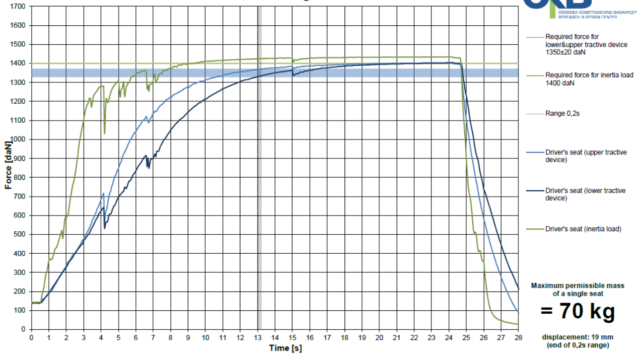
Original driver's seat with swivel OB-C on original seat base, Volkswagen Crafter/MAN TGE, M1
