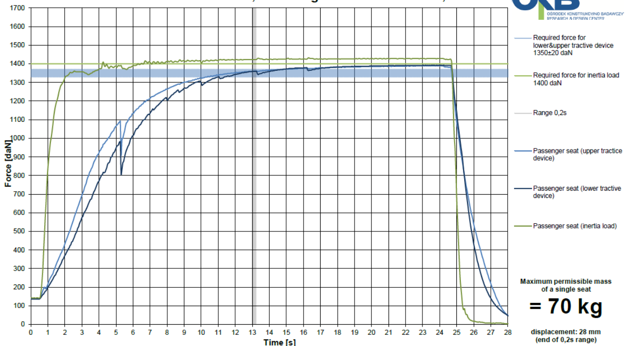
Original passenger seat with swivel OB-C on original seat base, Volkswagen Crafter/MAN TGE, M1
